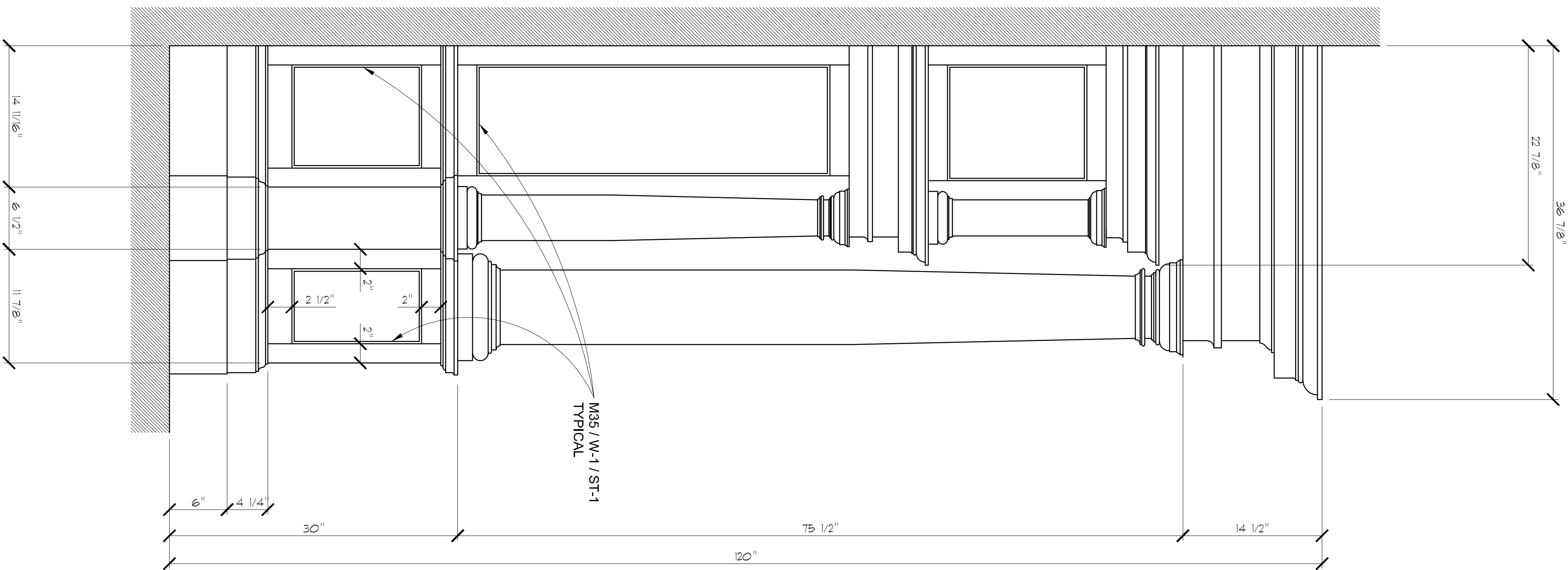
SIDE ELEV 1 FAMILY ROOM - TV CABINET ROOM No. FAMILY ARCH REF: 3/AS09 & A917 SCALE: 1/2" = 1'-0" RECD. 1
