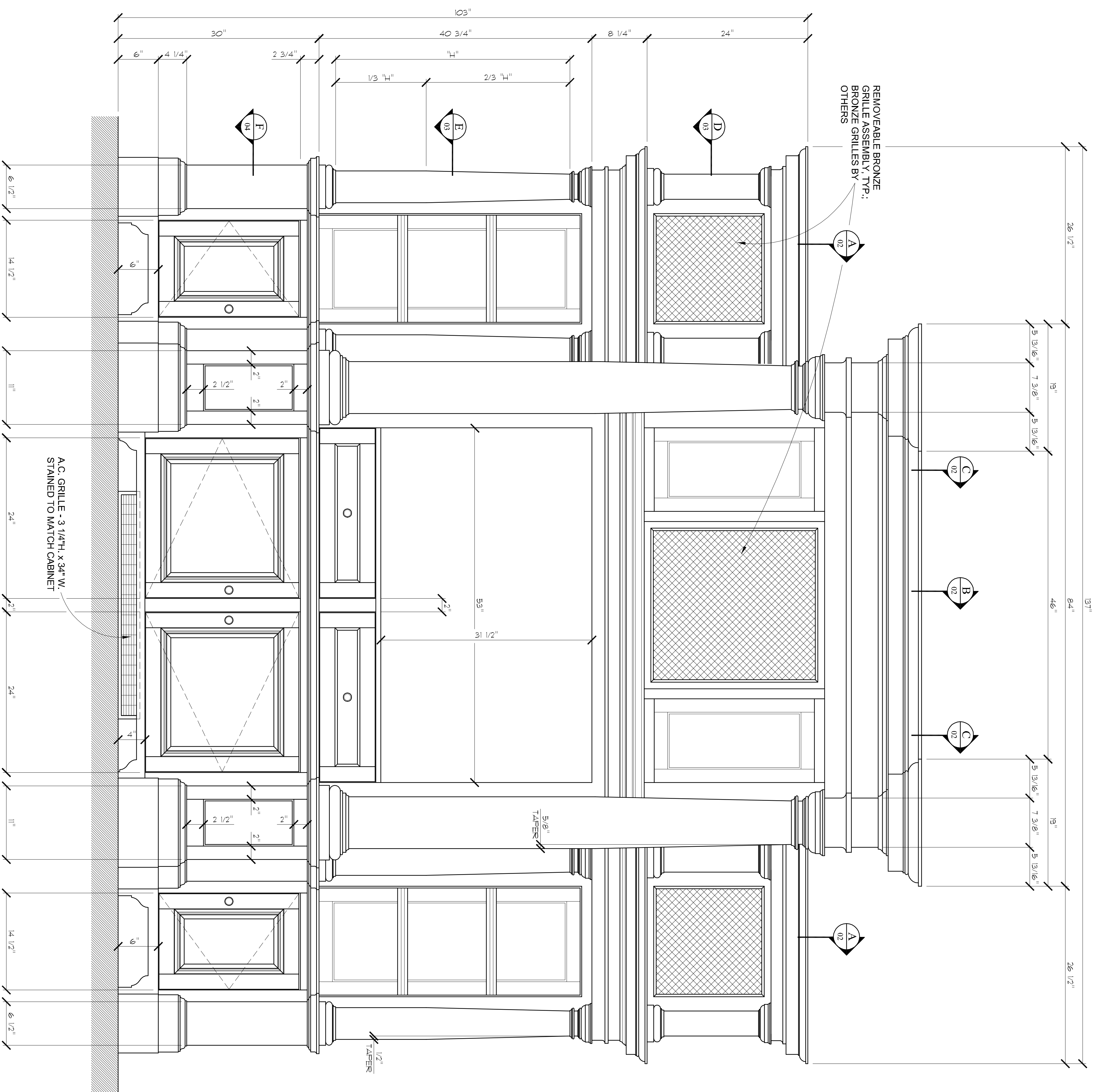
ELEVATION 2 FAMILY ROOM - TV CABINET ROOM No. FAMILY ARCH REF: 2/AS09 & A917 SCALE: 1/2" = 1'-0" RECD. 1
